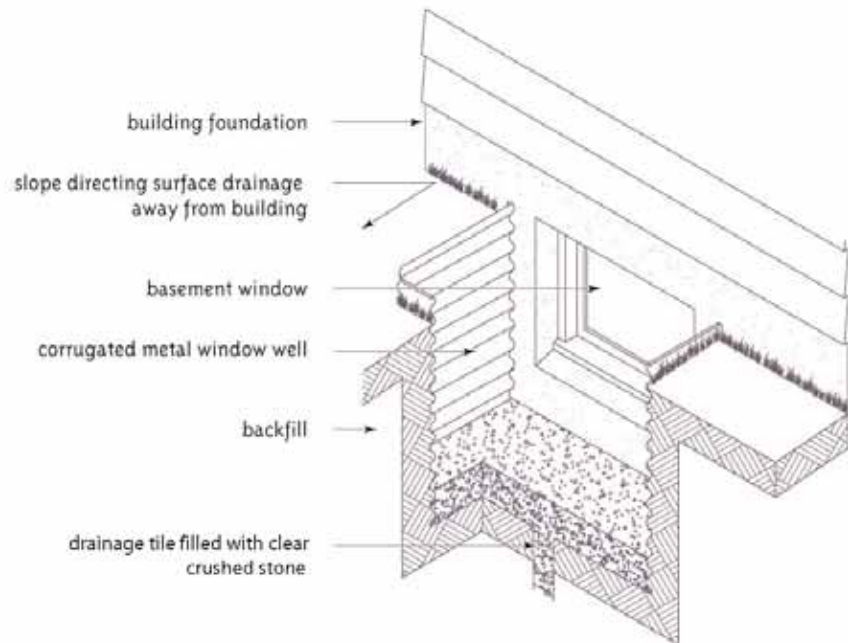
Figure 2: Window well at basement wall
