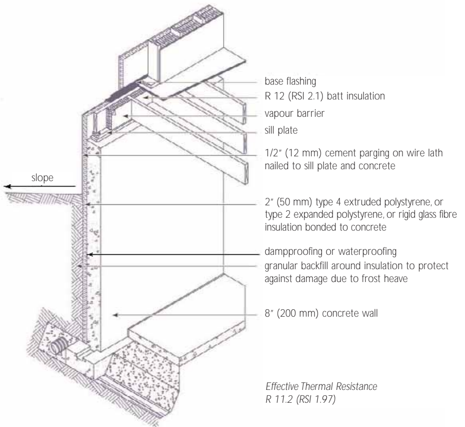
Figure 1: Concrete foundation wall with insulated exterior face
